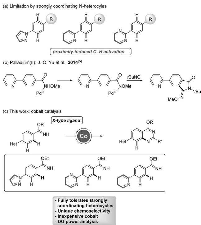
Figure 1. C–H activation in the presence of strongly coordinating heterocycles. a) Challenges. b) Palladium(II) catalysis. [5] c) Heterocycle-tolerating cobalt catalysis.
